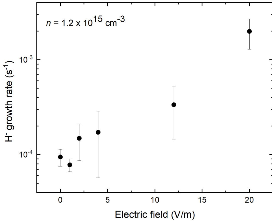
Extended Data Fig. 2 | Ion trap simulations including stray electric fields. Numerical simulations of the expected reaction rates at a hydrogen gas density of 1.2 \times 10^{15} \text{ cm}^{-3} , with error bars as in Fig. 3a. The electric fields were chosen to be homogeneous and oriented in one direction perpendicular to the RF
