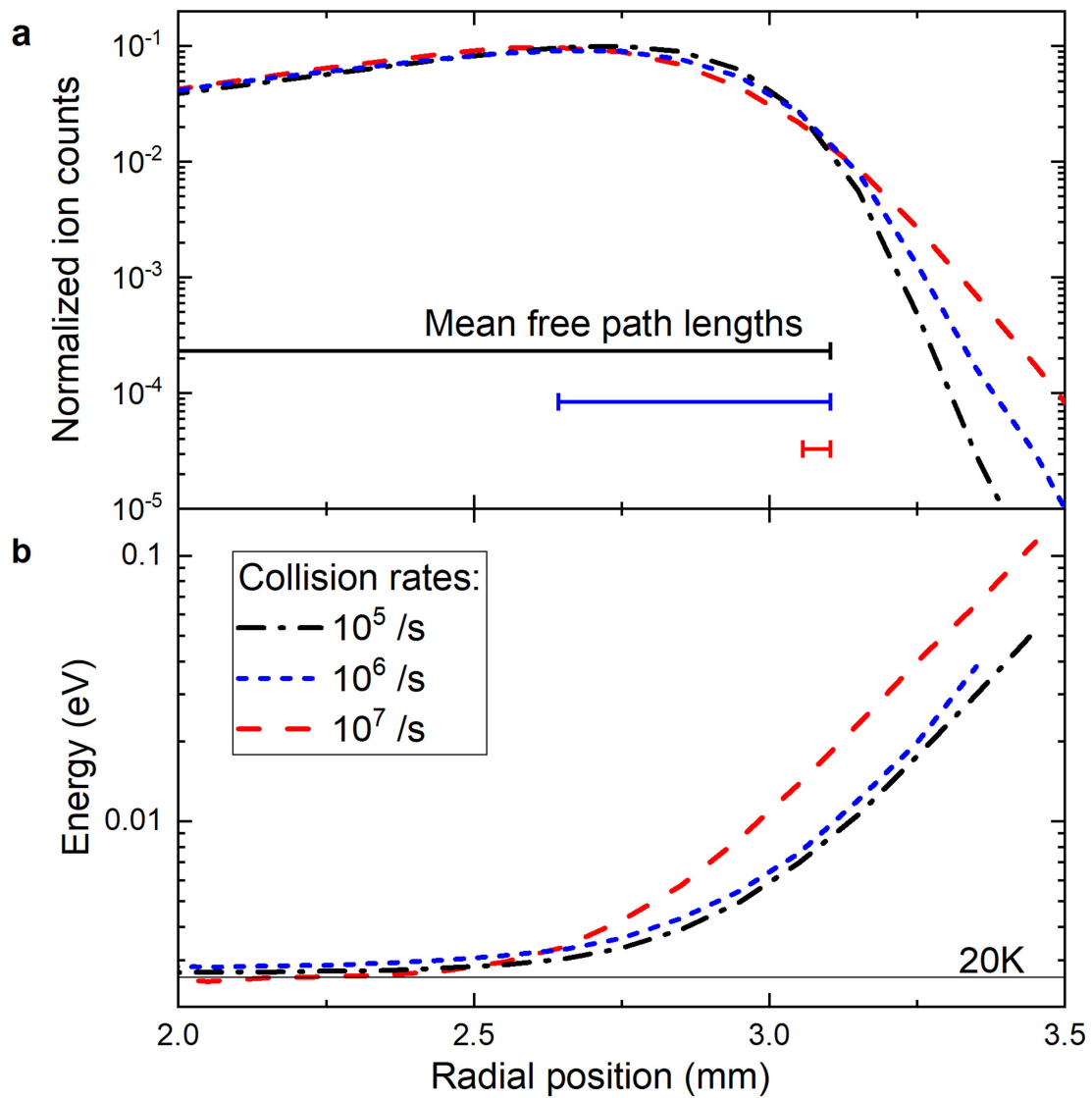
Extended Data Fig. 1 | Ion trap simulations for different densities. Distributions of ion number and energy as a function of the radial position in the trap, at different collision rates and with a buffer gas temperature of 20 K. a With higher collision rates, ions move, on average, slightly closer to the centre, but also increase in number at large radii. Mean free path lengths are
